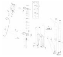
FORK
