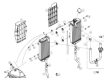
RADIATOR
