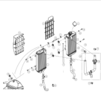
RADIATOR
