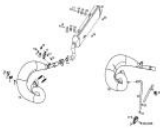
EXHAUST SYSTEM
