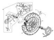
REAR WHEEL
