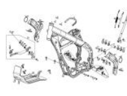
FRAME
