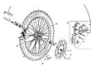
FRONT WHEEL
