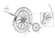
FRONT WHEEL
