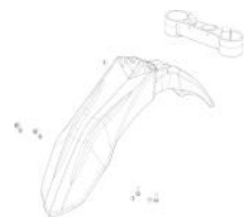
FRONT FENDER
