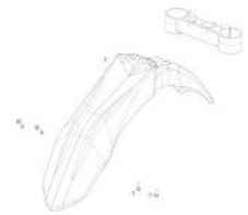
FRONT FENDER
