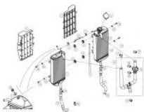
RADIATOR
