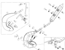
EXHAUST SYSTEM
