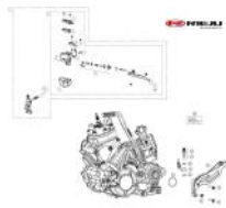
CLUTCH CONTROL
