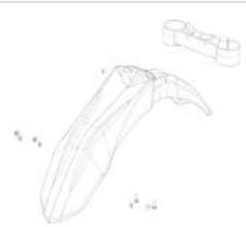
FRONT FENDER
