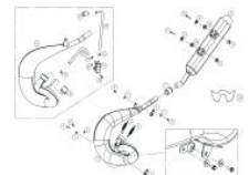
EXHAUST SYSTEM
