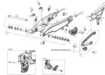
SWINGARM
