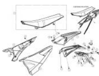
REAR FAIRING
