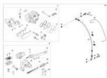
FRONT BRAKE
