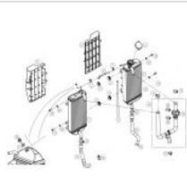
RADIATOR
