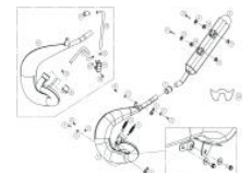
EXHAUST SYSTEM
