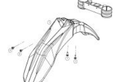
FRONT FENDER
