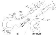
EXHAUST SYSTEM
