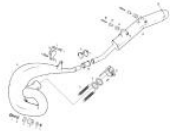
EXHAUST SYSTEM
