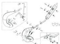
EXHAUST SYSTEM
