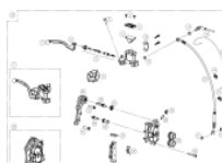
FRONT BRAKE
