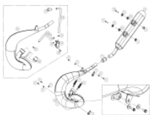
EXHAUST SYSTEM
